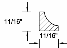
#2315 INSIDE CORNER
