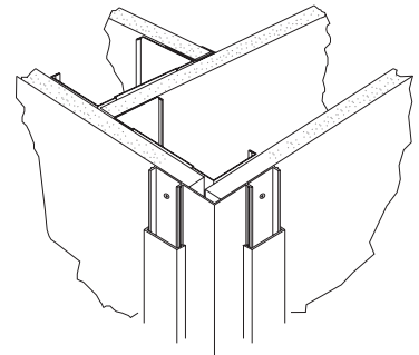
Surface corner
