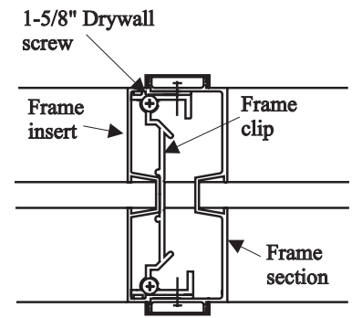
Detail of glazed post
