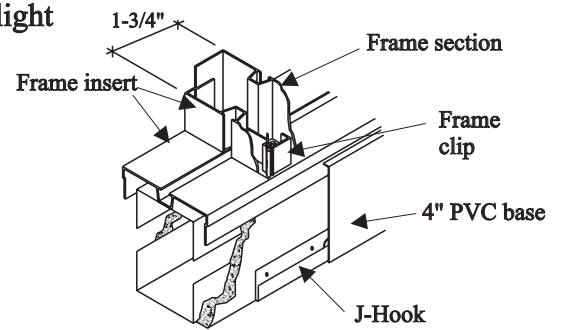
Glazed post at base sill
