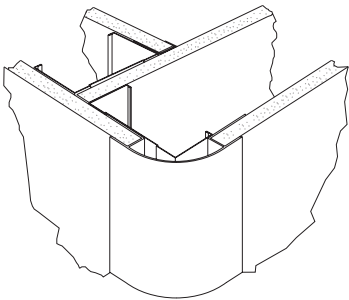
Round corner
